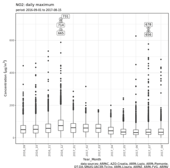
FIG. 2 BOX-AND-WHISKERS
